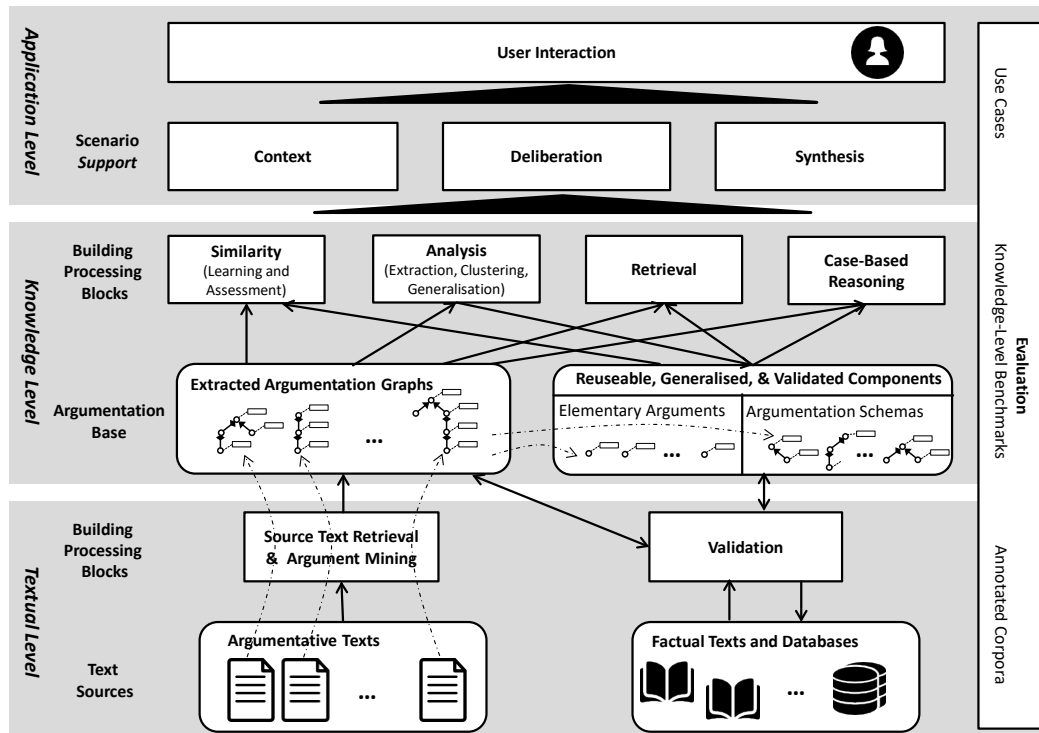
Fig. 2 Architecture of the argumentation machine.
